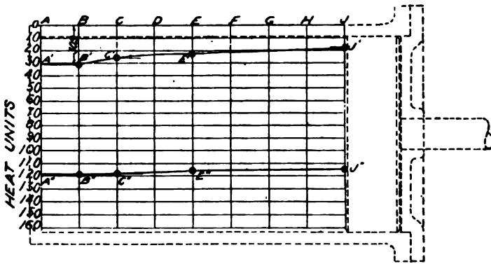
FIG. 230.—Diagram showing the number of heat units required to raise one-tenth pound of steam under the various pressures indicated by the position of the piston, at full stroke, half stroke and seven-eighths stroke. In using this diagram it is necessary to note that the heat units are calculated from -1^{\circ} Fahrenheit, instead of from 32^{\circ} , as is the general rule.
